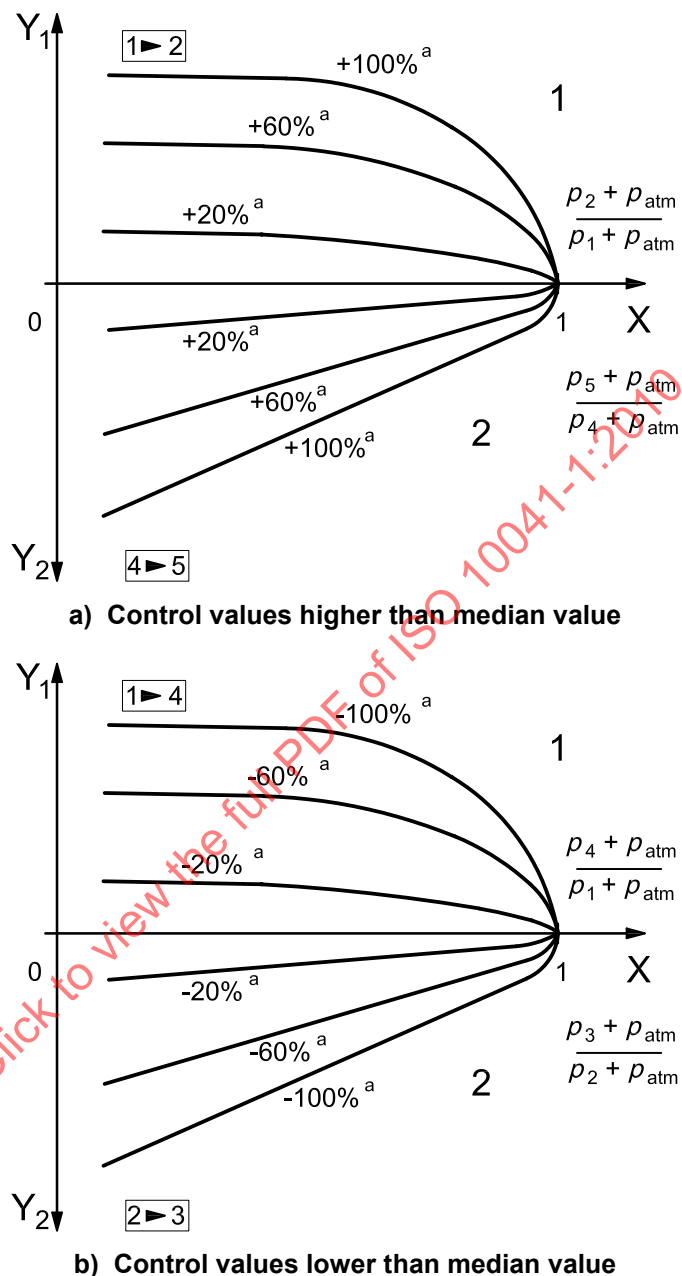
Figure 3 — Pressure-flow rate global characteristics in the case of a five-port control valve
