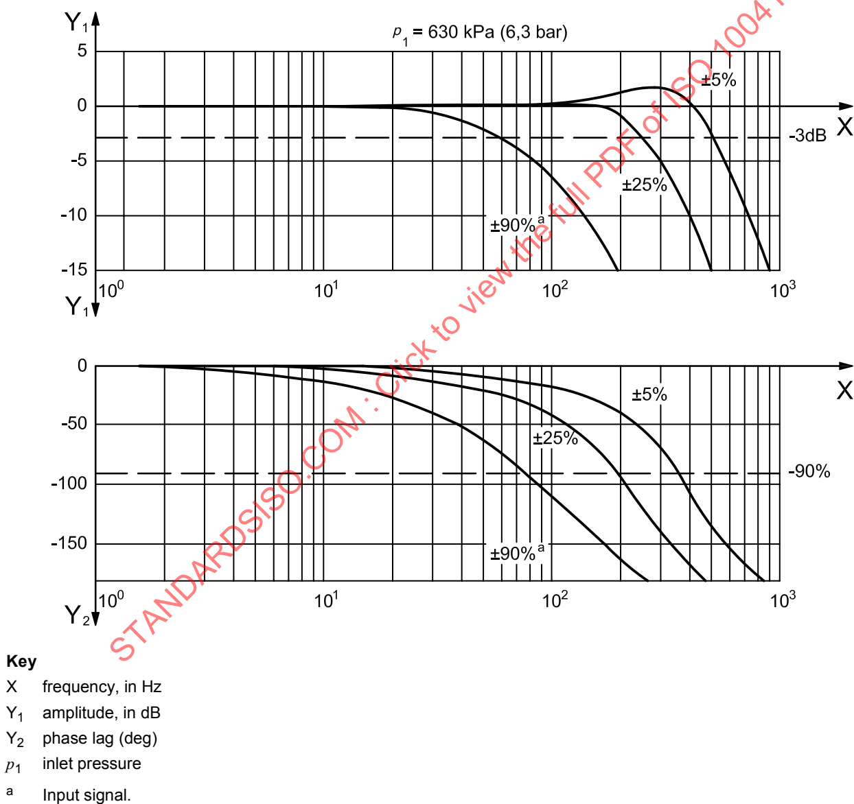
Figure 5 — Frequency responses
