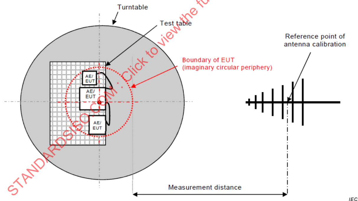
Figure 8 – Measurement distance
