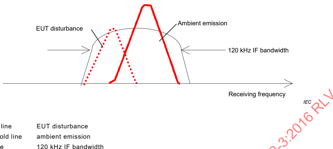
Figure A.3 – Disturbance by an unmodulated signal (dotted line)
