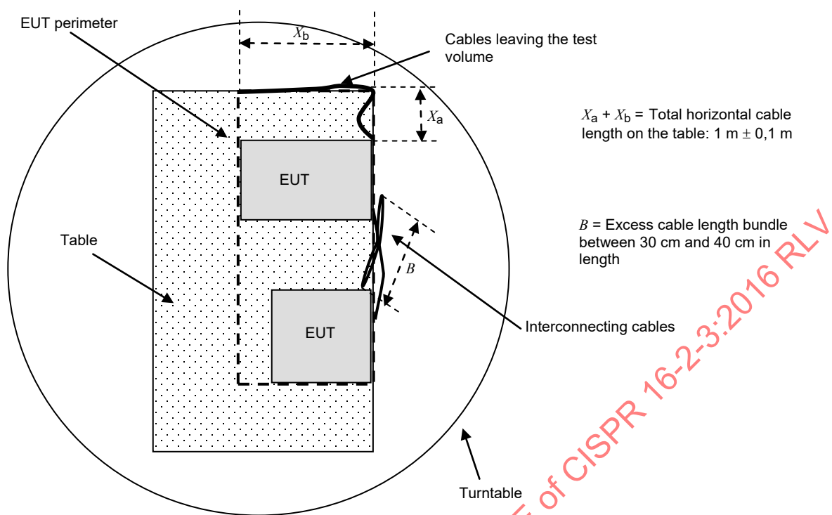
Figure 17 – Test set-up for table-top equipment – Top view
