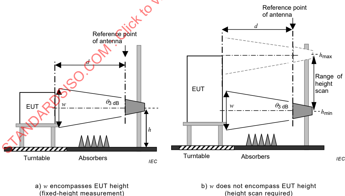
Figure 21 – Illustration of height scan requirements for two different categories of EUTs
