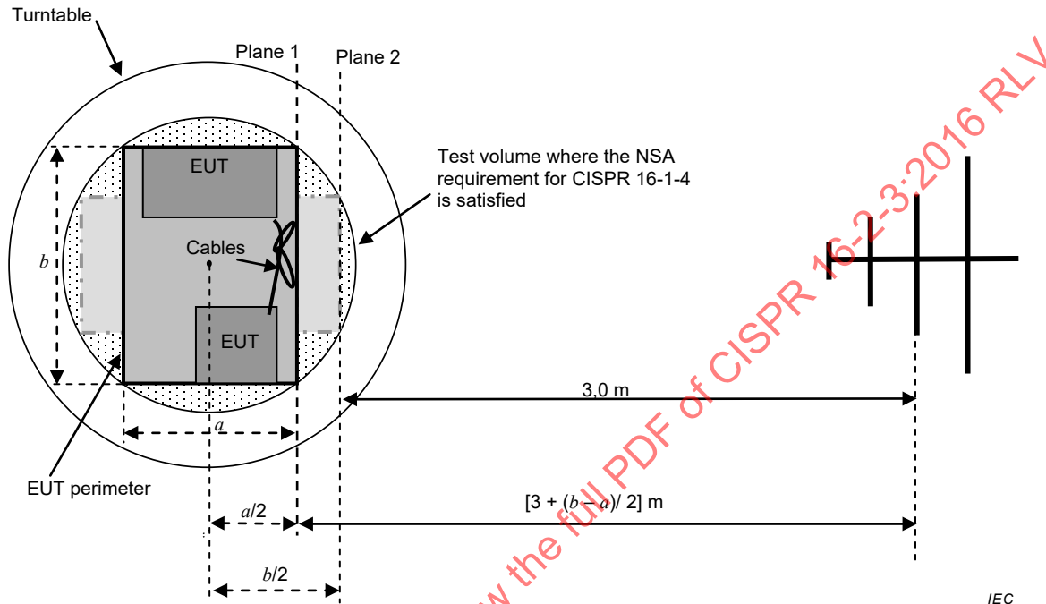
Figure 15 – Positions of reference planes for uniform field calibration (top-view)
