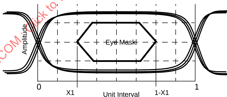
Figure 50 - Waveform eye mask
