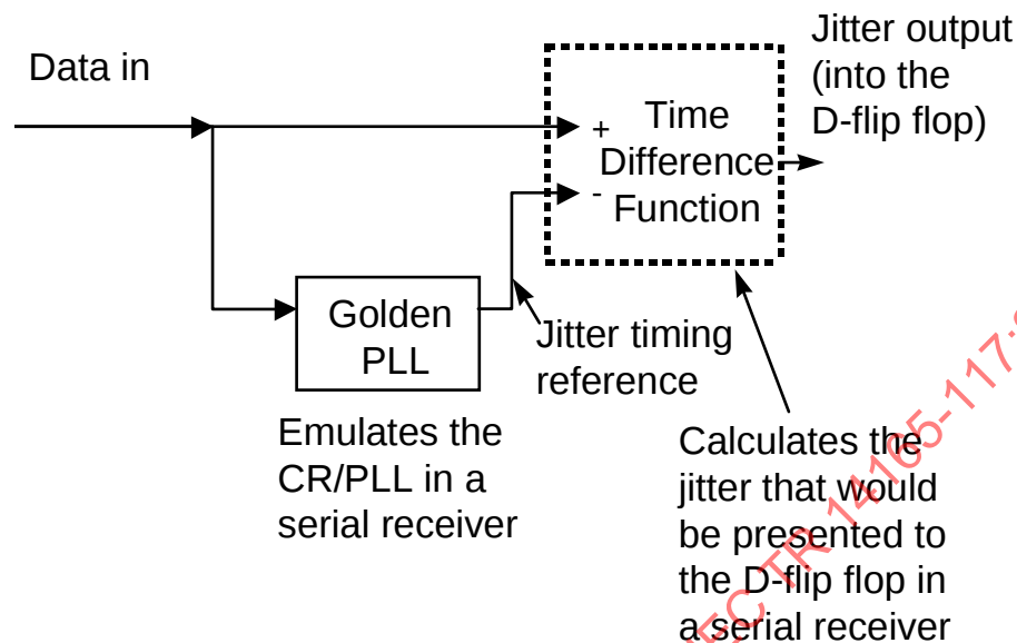
Figure 27 - Schematic of a basic measurement system
