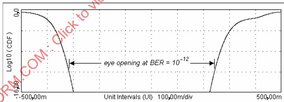
Figure 74 - Jitter analysis bathtub curve
