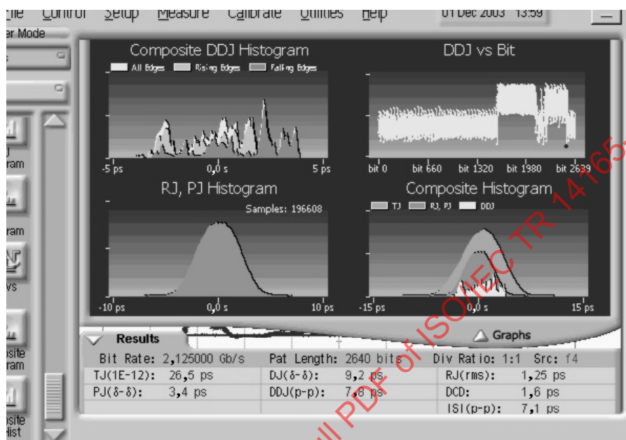
Figure 107 - CJTPAT Electrical Gamma T results
