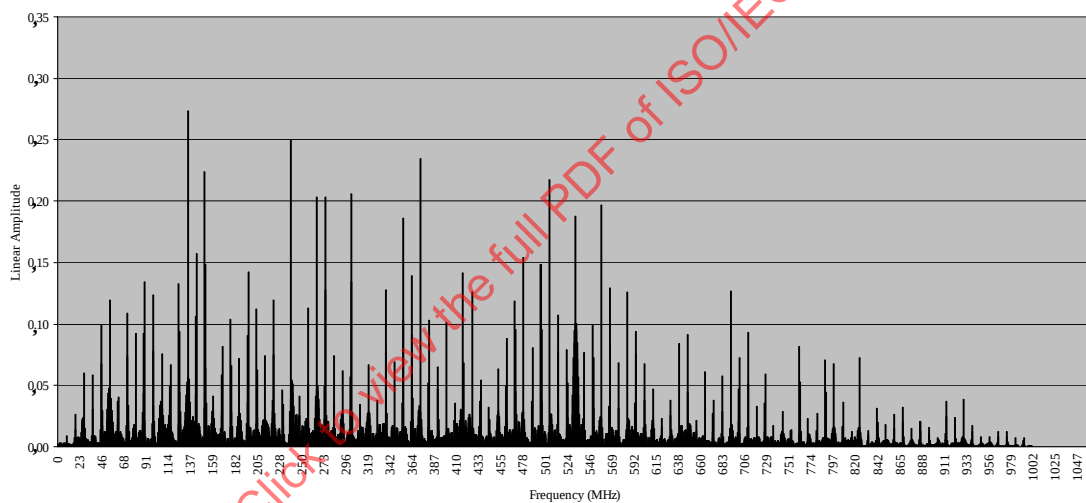
Figure A.3 - FFT of compliant RPAT
