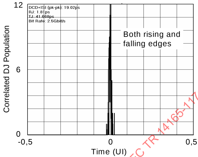
Figure 62 - Correlated DJ histogram measurement
