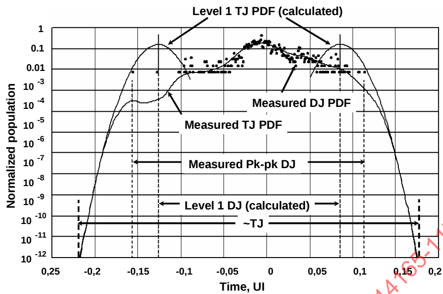
Figure 38 - Real data comparisons using PDFs
