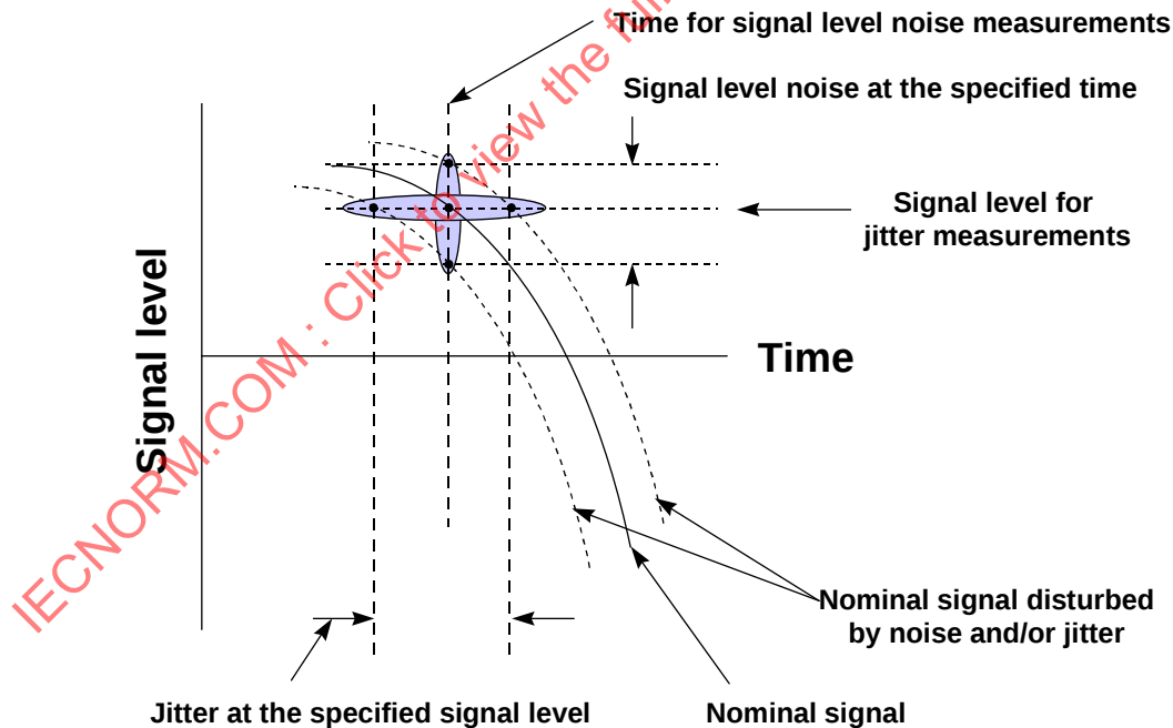
Figure 10 - Noise and jitter in the same portion of the signal
