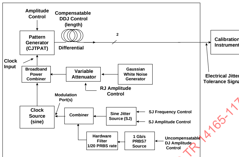
Figure 78 - Example of an electrical signal tolerance source
