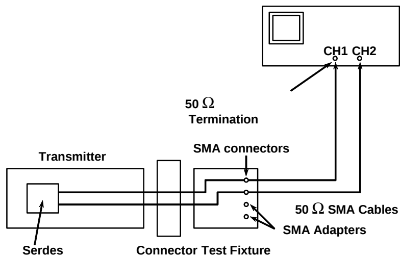
Figure 98 - Test fixture and termination Option 1
