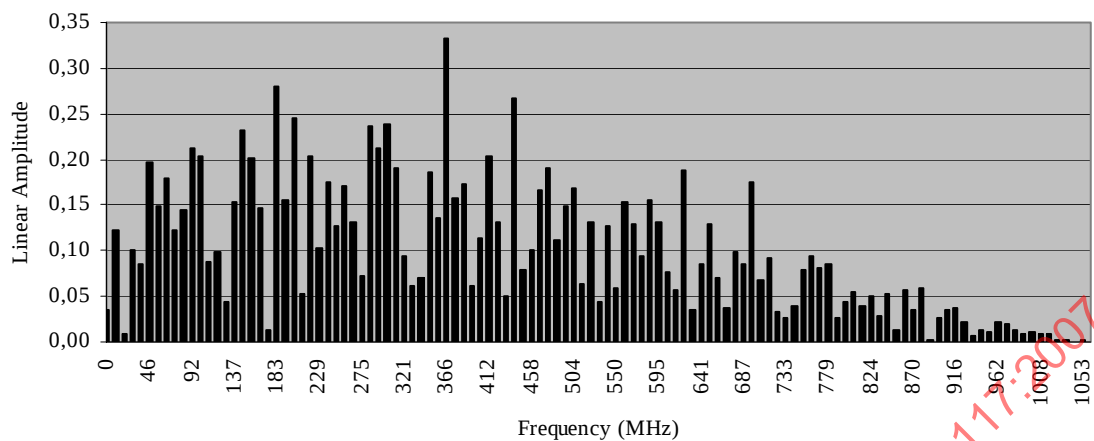
Figure A.2 - FFT of original RPAT
