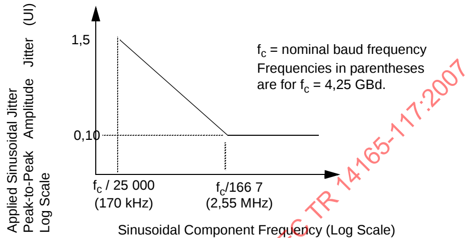
Figure 3 - Mask of the sinusoidal component of jitter tolerance - Log-Log Plot
