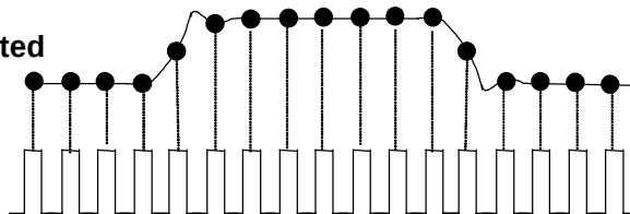
Figure 70 - Real-Time (RT) sampling (single trigger event)
