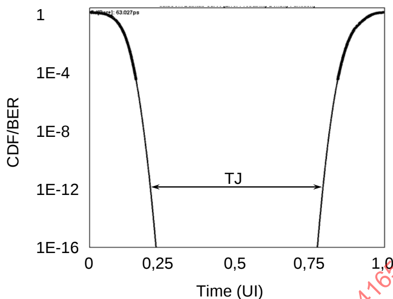
Figure 60 - BER/CDF function measured with “known pattern with marker method”
