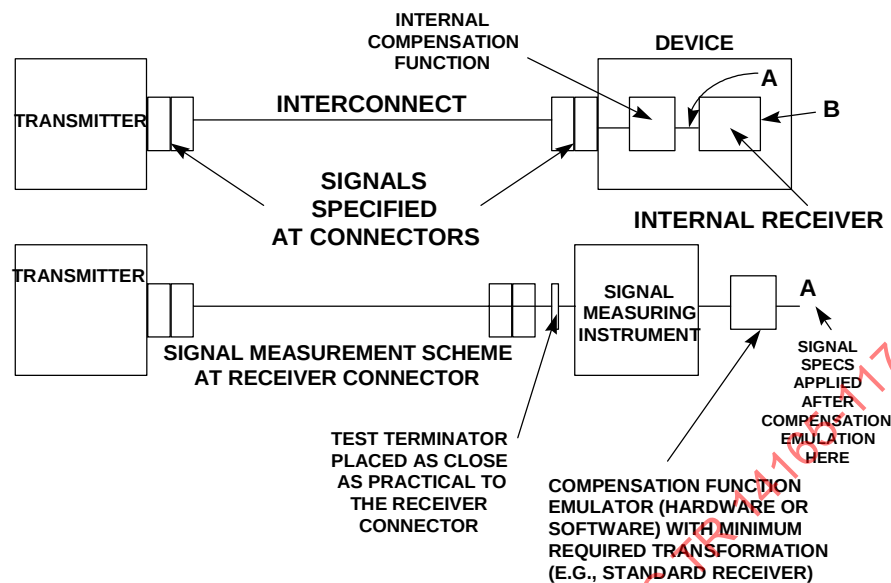
Figure 33 - Measurement set-up for evaluating receivers
