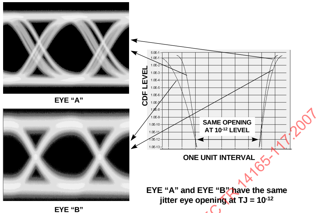
Figure 4 - Waveform eye diagrams from different jitter distributions
