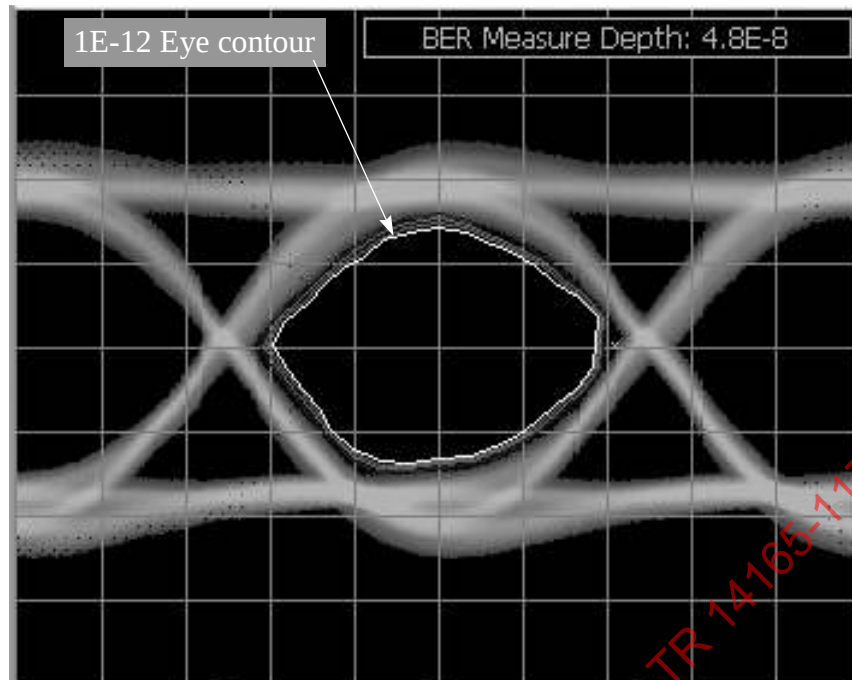
Figure 53 - Example of eye contour measurement and waveform eye
