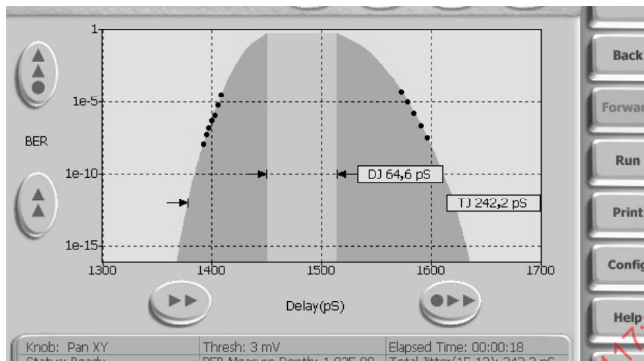
Figure 113 - Example of an automated BERT scan similar to figure 112
