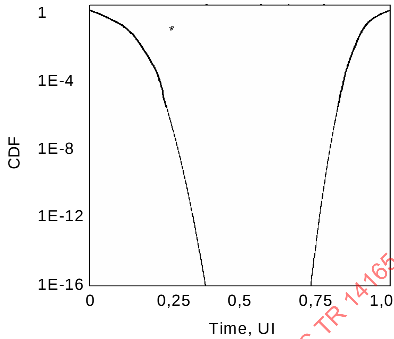
Figure 46 - Level 1 CDF “bathtub curve” for the PDFs in figure 45
