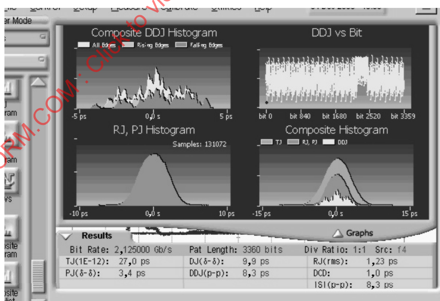
Figure 108 - Electrical Gamma T CRPAT results
