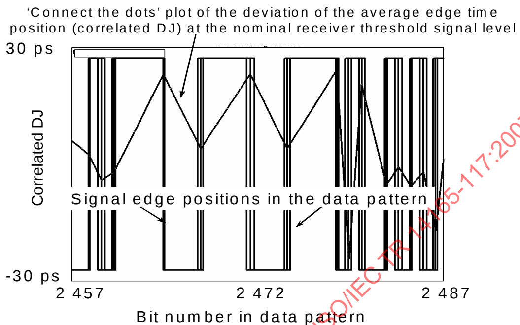
Figure 58 - Correlated DJ distribution as a function of bit number
