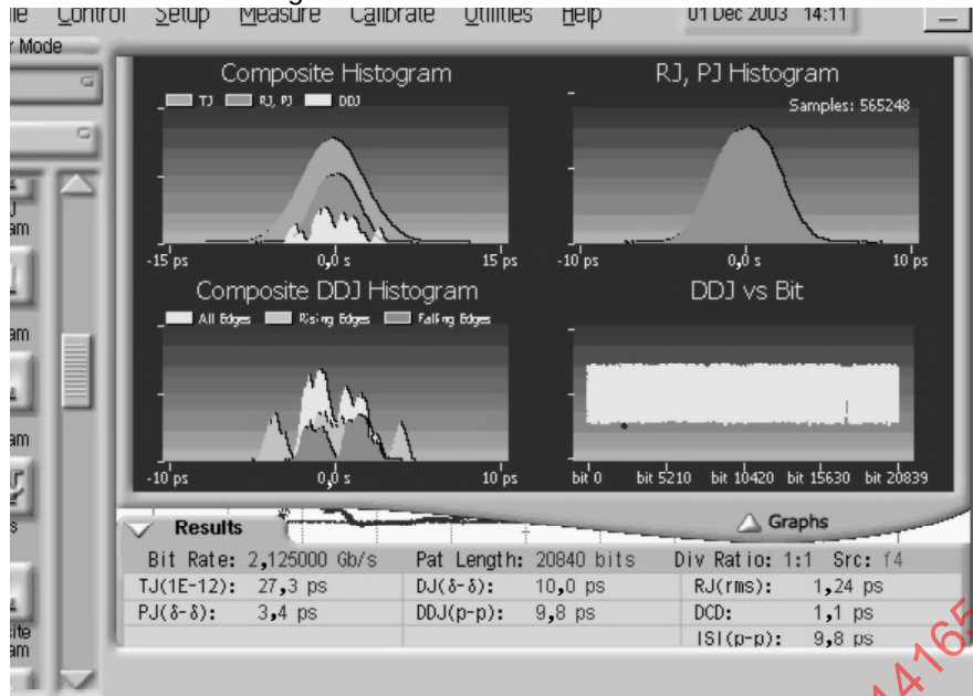
Figure 109 - Electrical Gamma T CSPAT results
