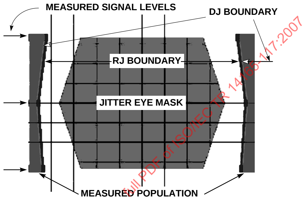
Figure 24 - Practical example using a TIA at three different signal levels
