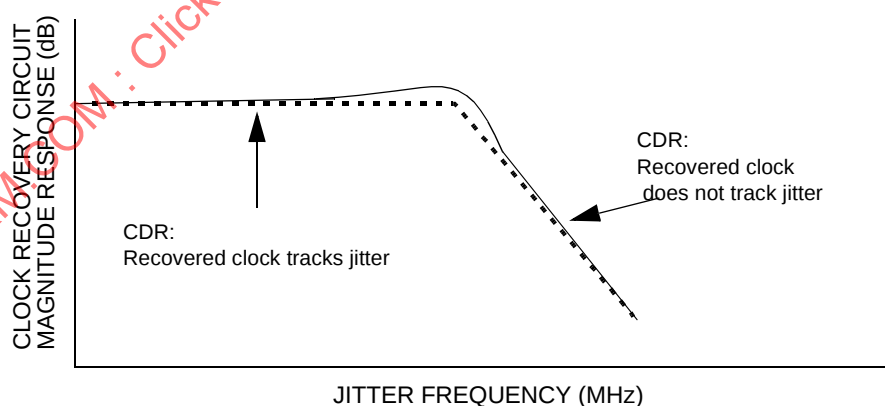
Figure 2 - PLL response
