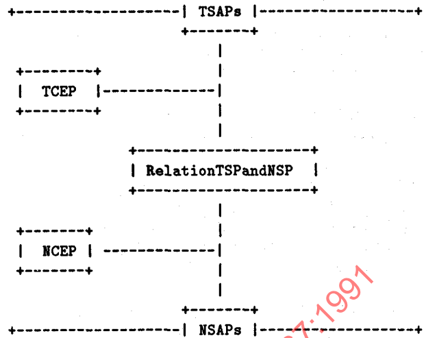
Figure 11.17: Decomposition of Process TPEConnection
