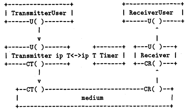
Figure 9.3: Architecture of the Sliding Window Protocol in Estelle
