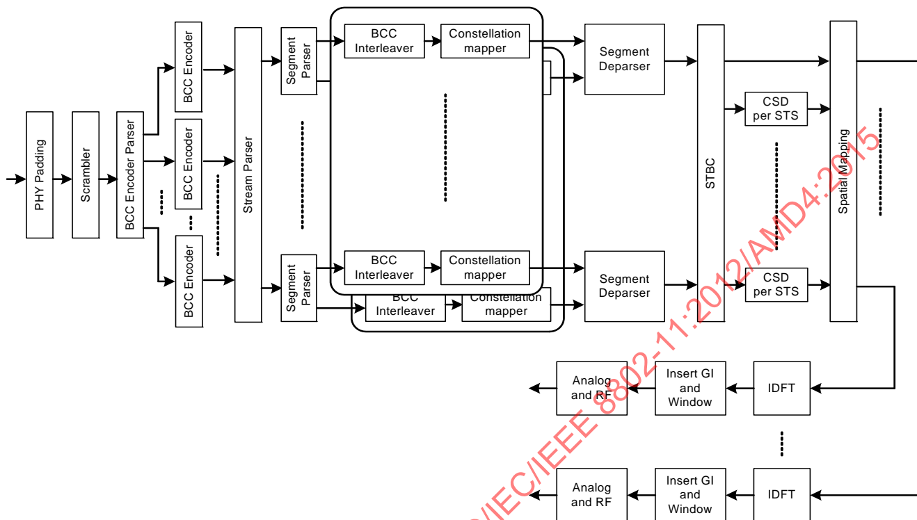
Figure 22-13—Transmitter block diagram for the Data field of a 160 MHz VHT SU PPDU with BCC encoding
