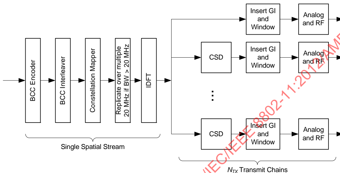
Figure 22-5—Transmitter block diagram for the L-SIG and VHT-SIG-A fields
