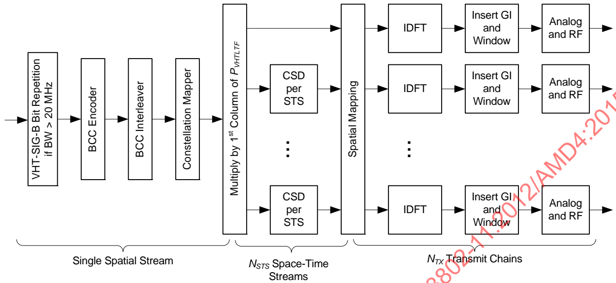
Figure 22-6—Transmitter block diagram for the VHT-SIG-B field of a 20 MHz, 40 MHz, and 80 MHz VHT SU PPDU
