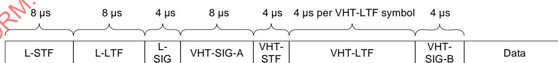
Figure 22-4—VHT PPDU format
