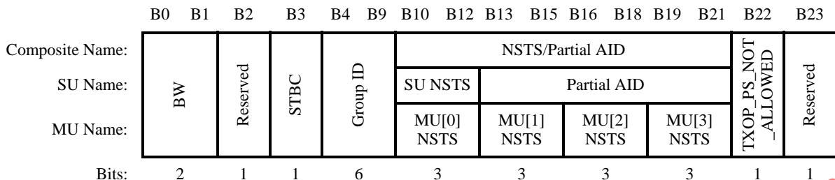
Figure 22-18—VHT-SIG-A1 structure
