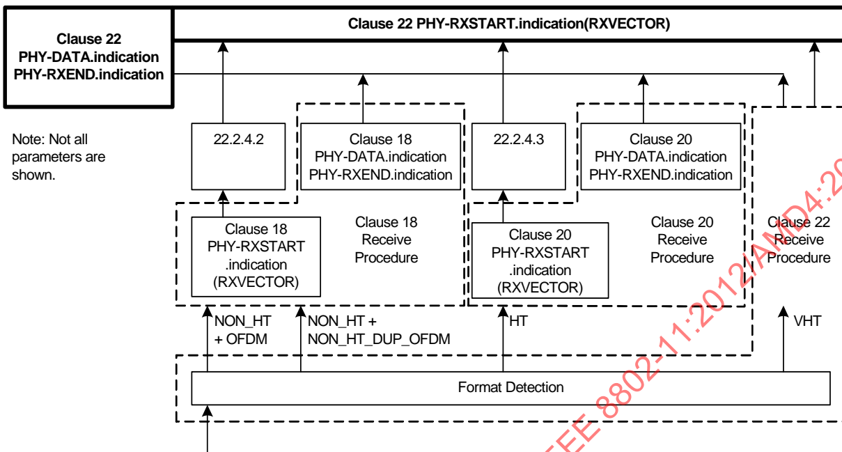
Figure 22-2—PHY interaction on receive for various PDU formats
