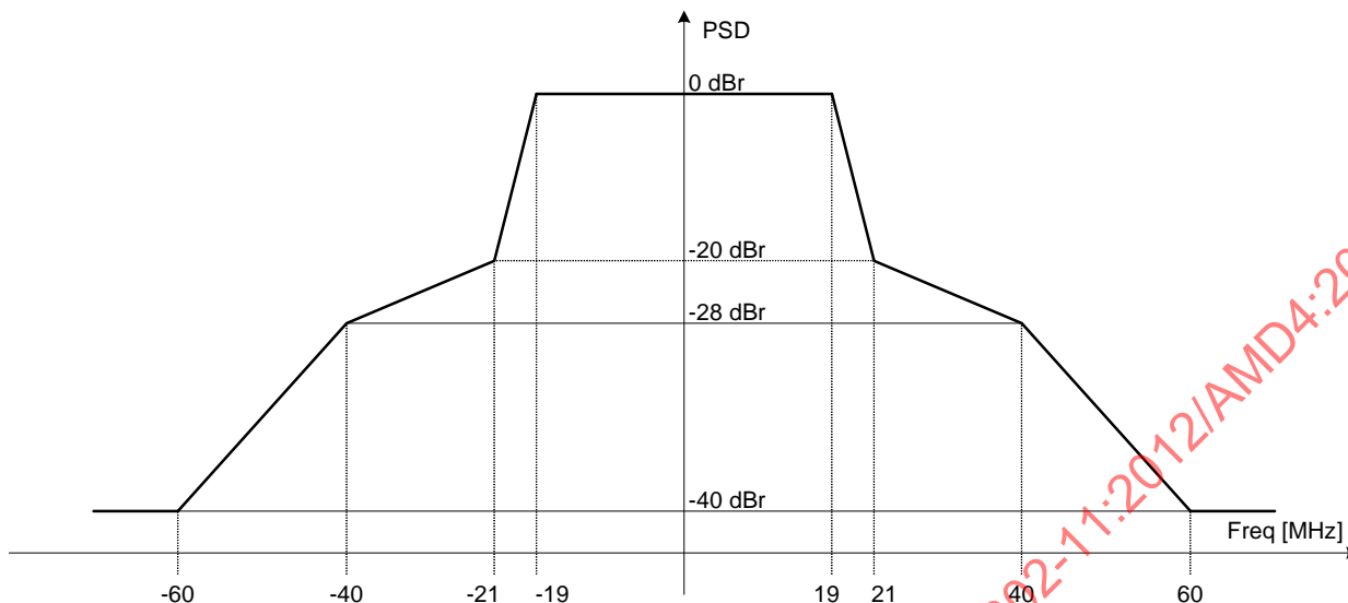
Figure 22-30—Example transmit spectral mask for a 40 MHz mask PDU
