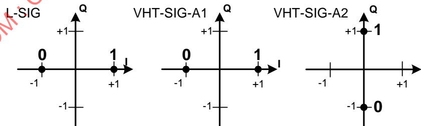
Figure 22-20—Data tone constellation in the VHT PDU pre-VHT modulated fields
