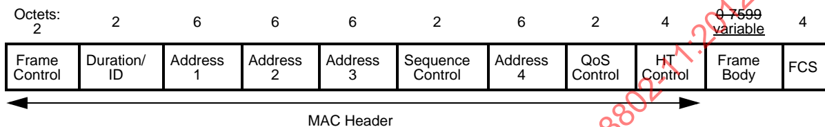
Figure 8-30—Data frame
