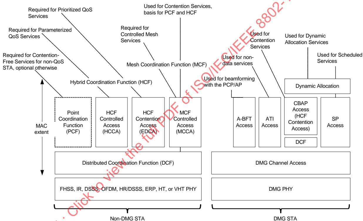
Figure 9-1—MAC architecture
