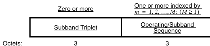
Figure 8-90c—Triplet field if dot11OperatingClassRequired is true
