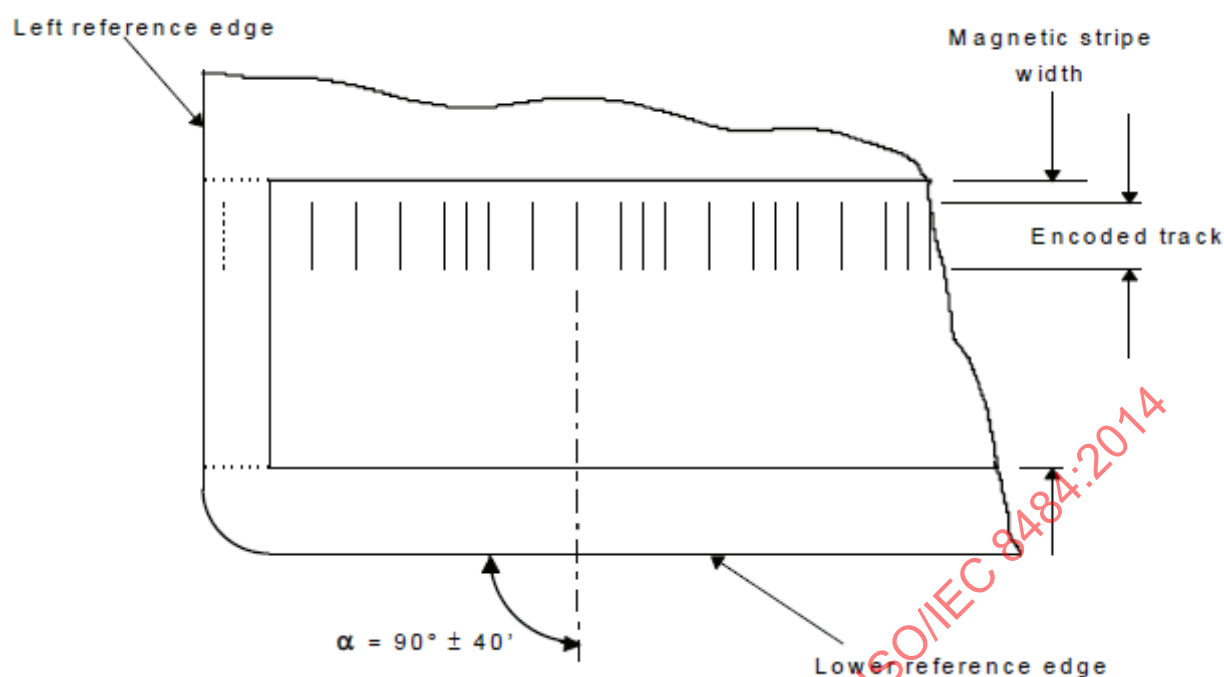
Figure 7 — Angle of recording
