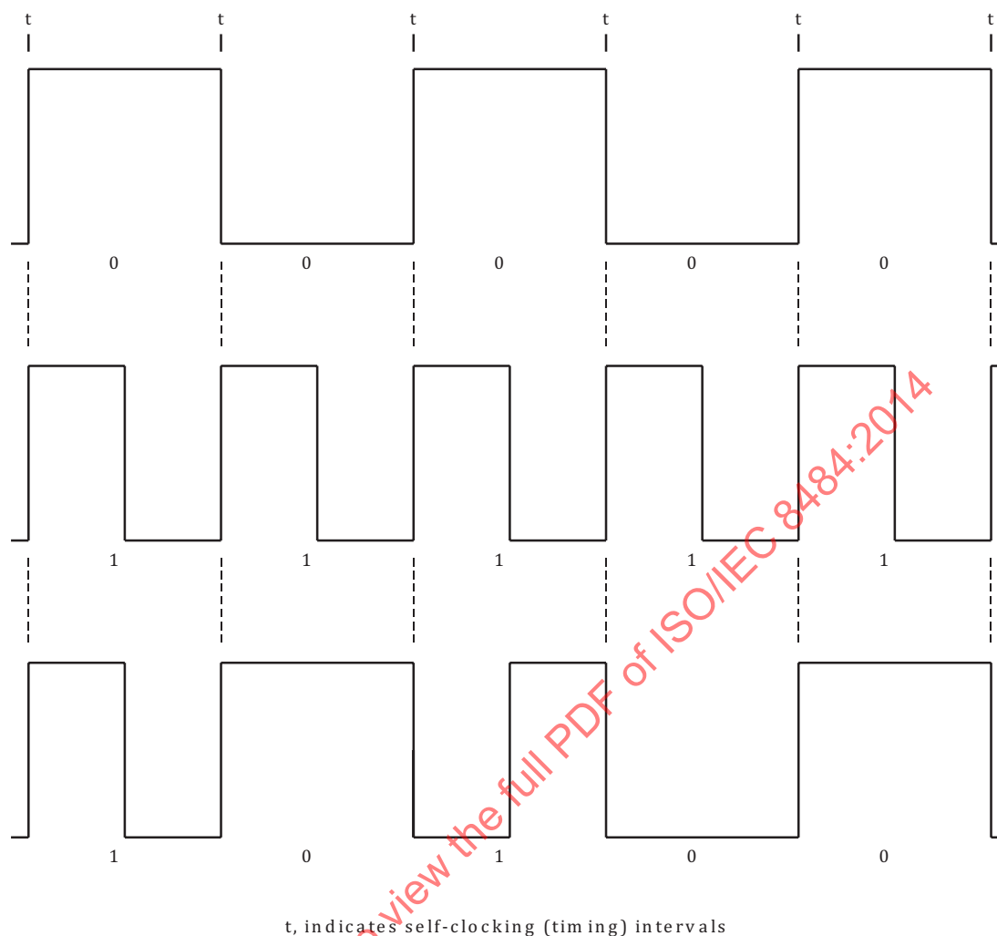
Figure 6 — Examples of two-frequency encoding
