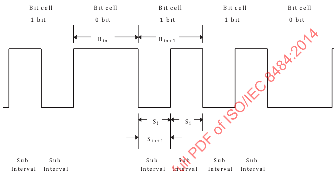
Figure 8 — Flux transition spacing variation
