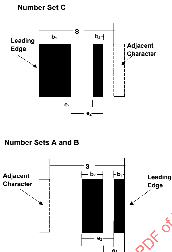
Figure 7 — Symbol character decode measurements
