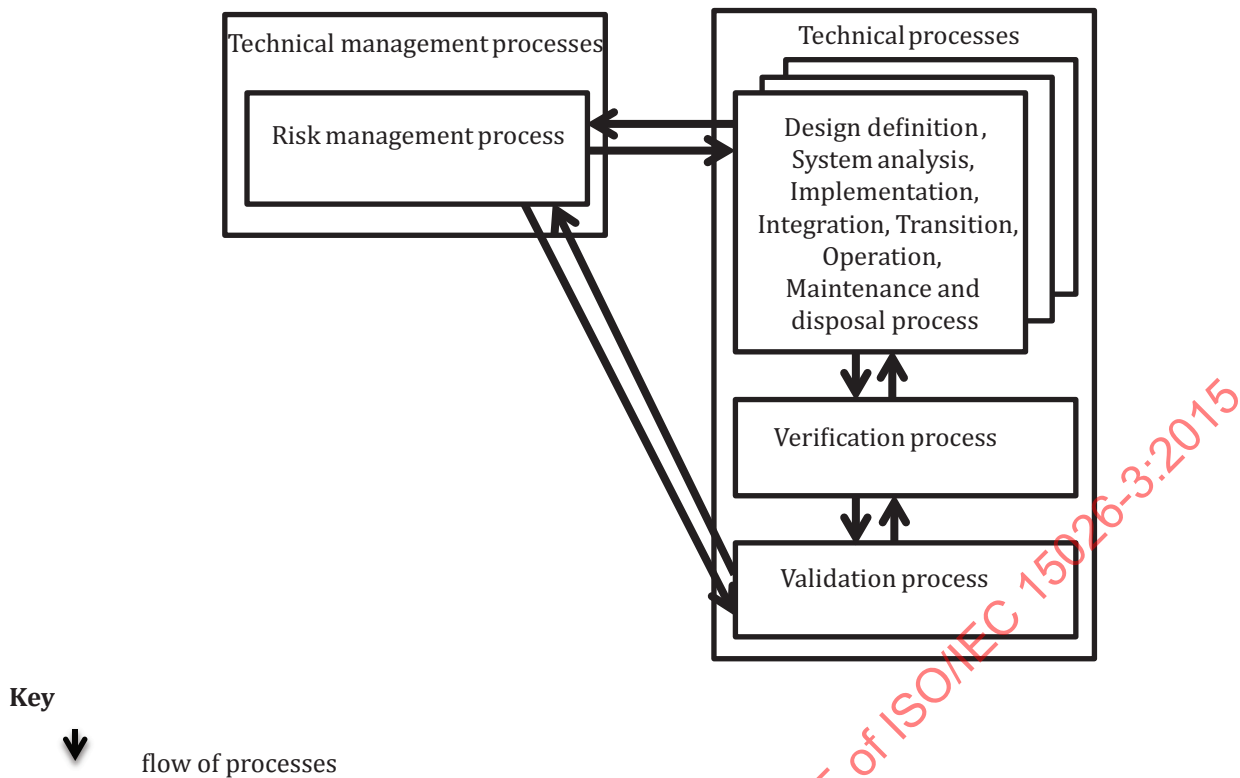
Figure 7 — Related processes in ISO/IEC/IEEE 15288 to the process of meeting integrity level requirements (informative)
