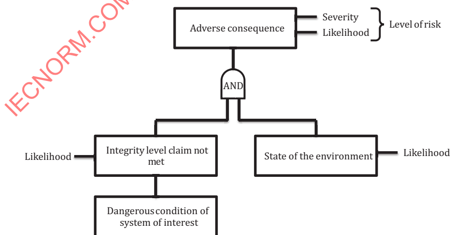
Figure 3 — Relationship between adverse consequence, state of the environment and integrity level claim (informative)
