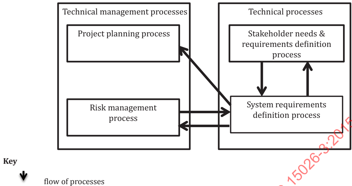
Figure 5 — Related processes in ISO/IEC/IEEE 15288 to the system integrity level determination process (informative)
