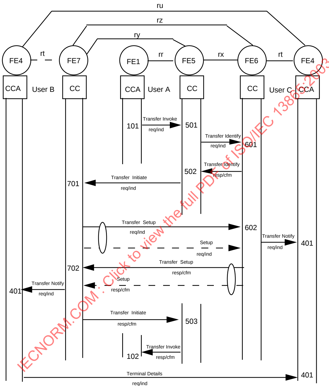
Figure 12 - Information Flow Sequence - Normal Operation of SS-CT (User C answered)
