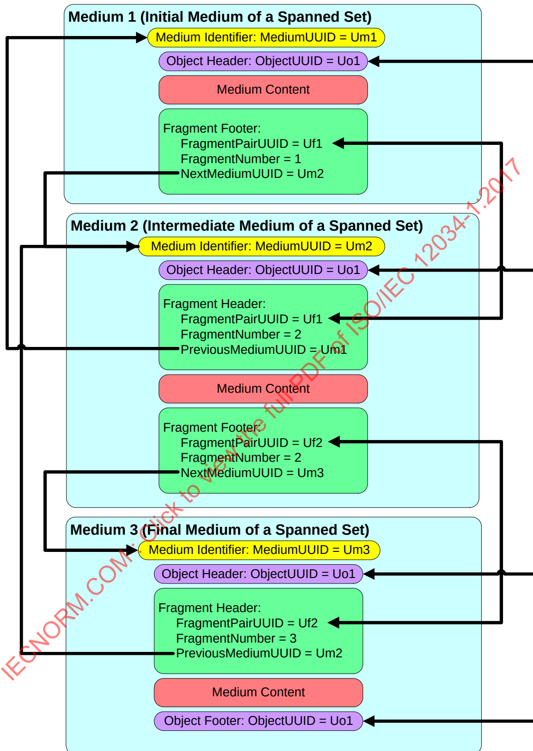
Figure 6 – Linkages between Fragments of a Spanned Set
