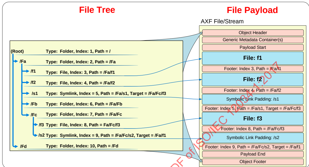
Figure 5 – File Tree Structure Overview
