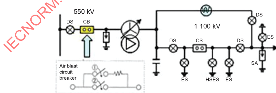
Figure B.1 – Circuit for transient voltage and current measurement
