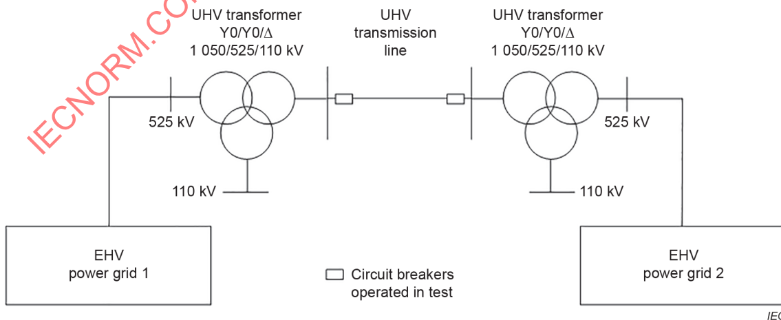
A.3c – Interconnecting/splitting test operated by UHV transmission line circuit breakers to make two power grids of same voltage level run in/out of synchronous interconnection
