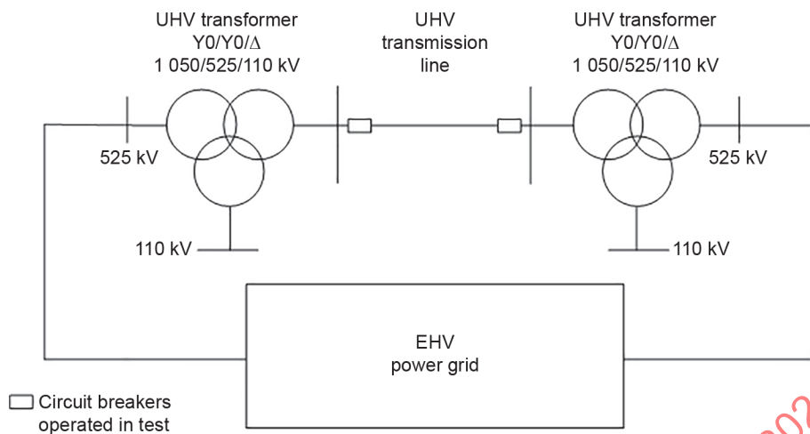
A.3a – Loop closing/opening test operated by UHV transmission line circuit breakers to make the power grid of different voltage levels run in/out of loop network
