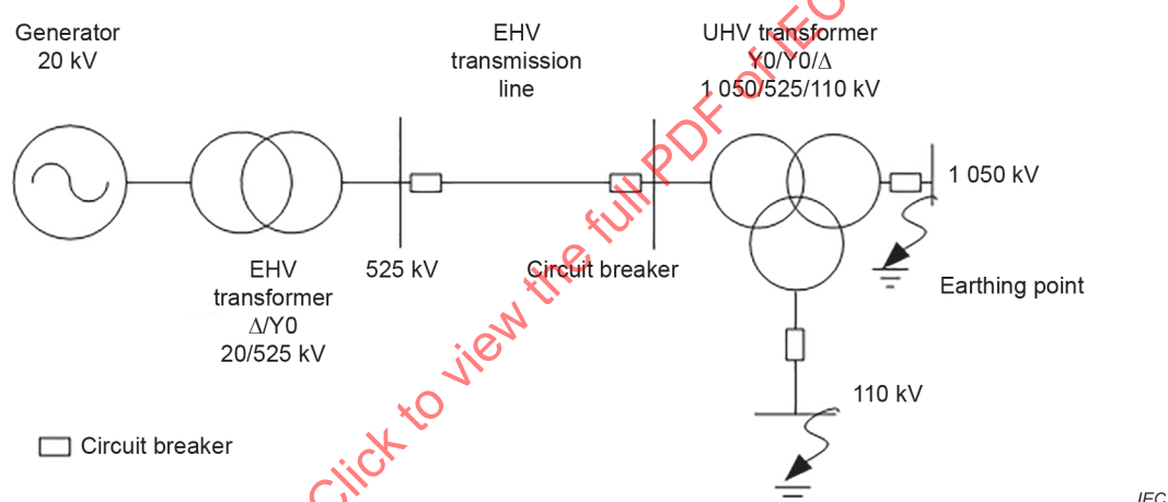
Figure A.1 – Circuit for test of UHV transformer with current increasing from zero
