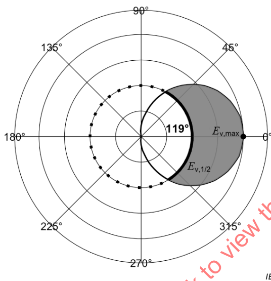
a) Suspended task light with horizontal FWHM = 119°
