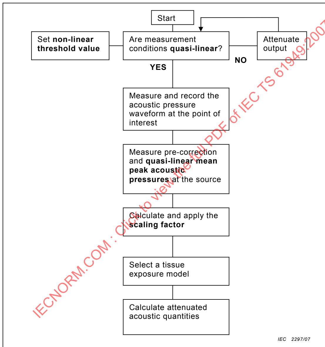
Figure 1 – Flow diagram for obtaining values of attenuated acoustic quantities
