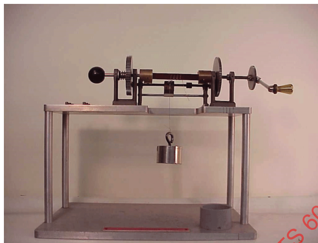
Figure 4 – Heater wire winding device (Example)
