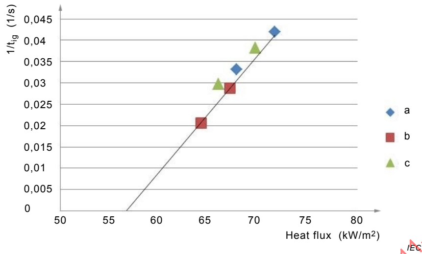
Figure C.5 – 1/t_{ig} for Material C
