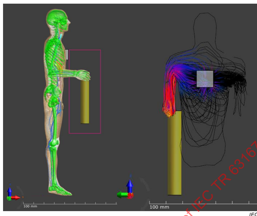
Figure 6 – Realistic computational 3D human body model and results of calculation of current density and pathway
