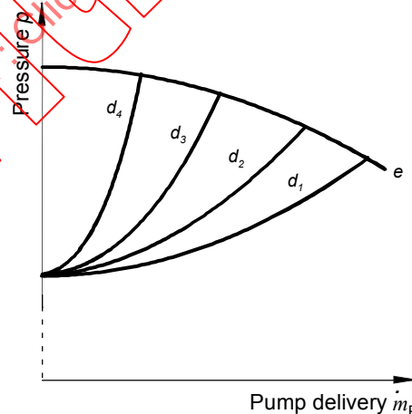
Figure 7 – Family of characteristics with throttling
