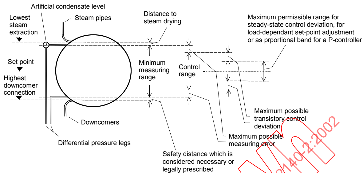
Figure 3 – Measuring and control ranges on the drum
