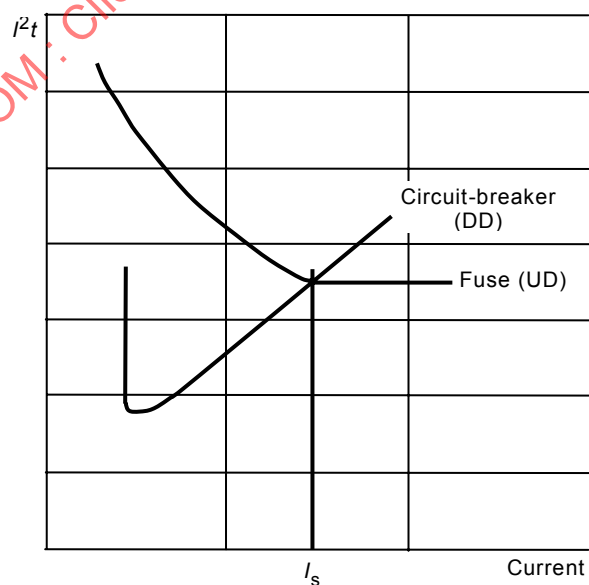
Figure 7 – FU/CB – Verification of selectivity between fuse and circuit-breaker for operating time t < 0,1 s
