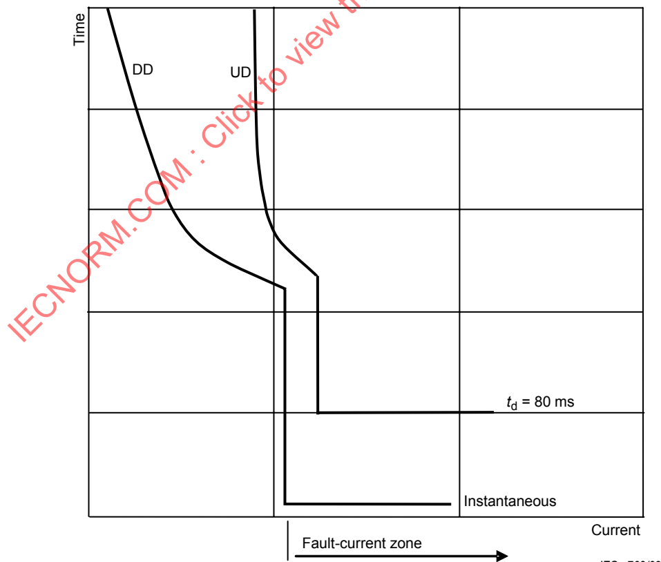
Figure 2 – Example of selectivity in the fault current zone with time-delay short-circuit release
