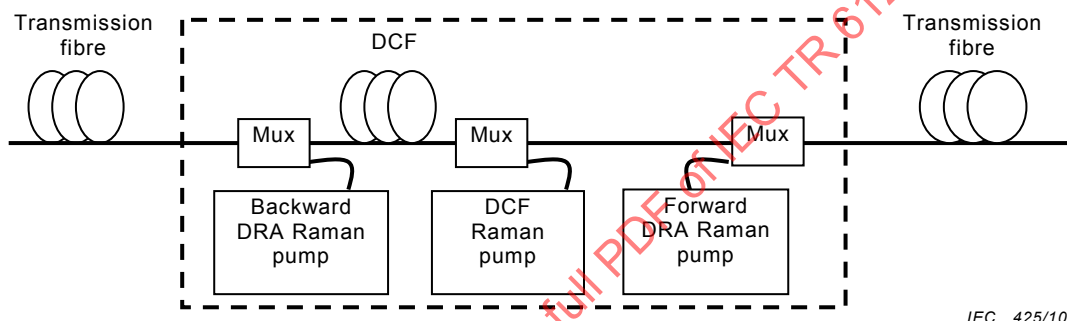
Figure 6 – Typical configuration of an amplification site in an all-Raman system
