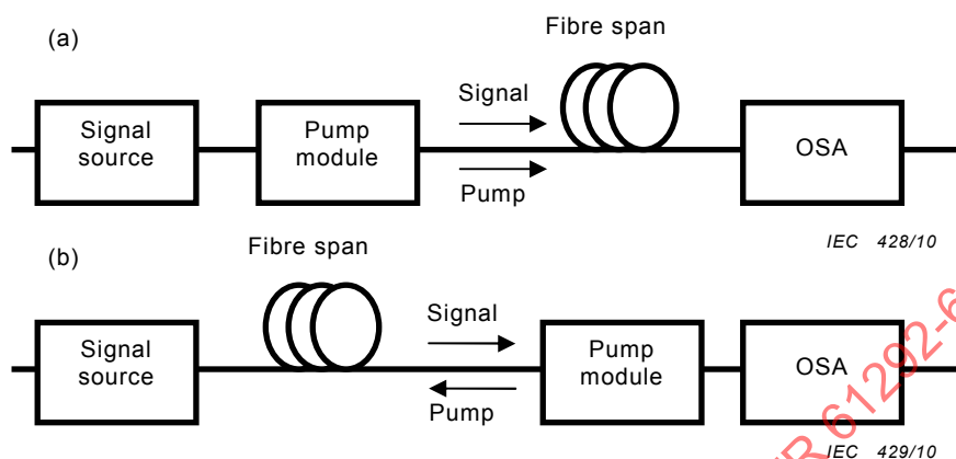
Figure 9 – Typical configuration used to measure on of gain (a) for co-propagating DRA and (b) for counter-propagating DRA
