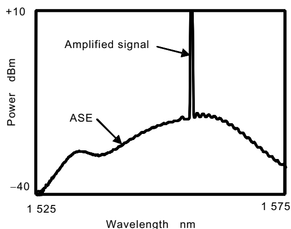
Figure 2 – Spectrum of optical fibre amplifier output
