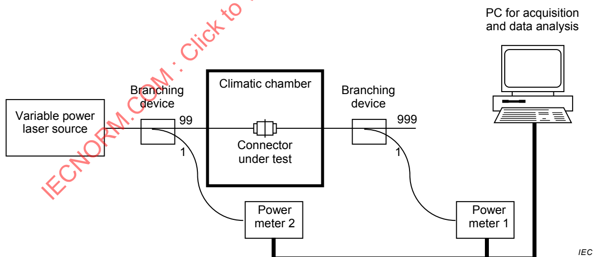
Figure 3 – Test set-up
