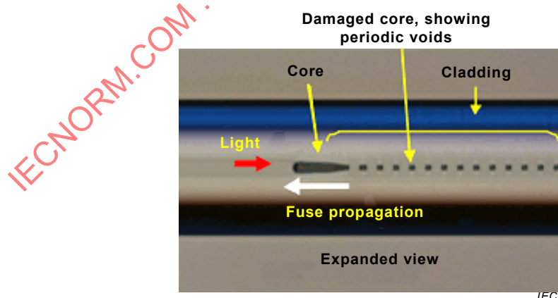
Figure A.1 – Front part of the fibre fuse damage generated in the optical fibre
