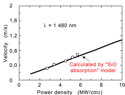
Figure A.6b – Propagation velocity at the wavelengths of 1 480 nm
