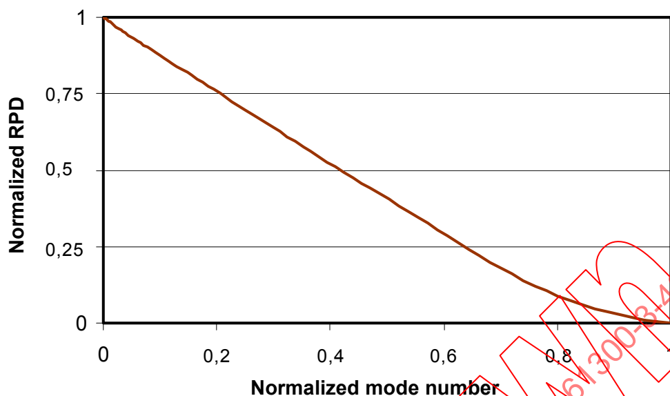
Figure 3 – Example of normalized RPD
