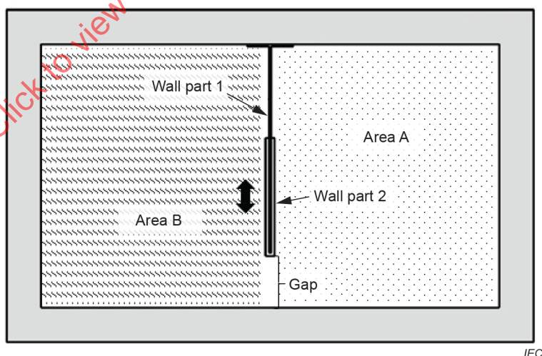
Figure 9 – Minimum passable gap width test
