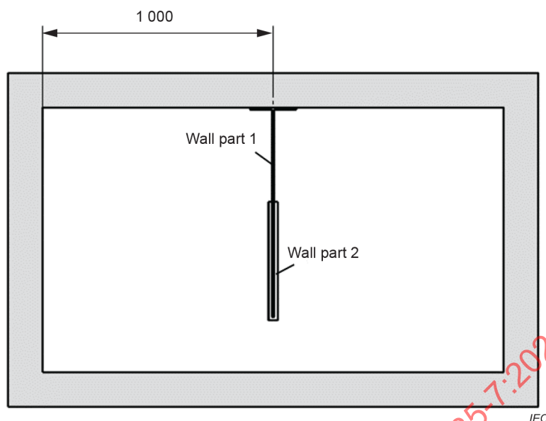
Figure 21 – Test bed with an additional adjustable wall
