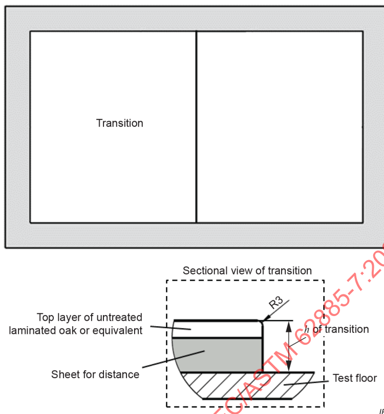
Figure 24 – Test bed with additional transition and its sectional view
