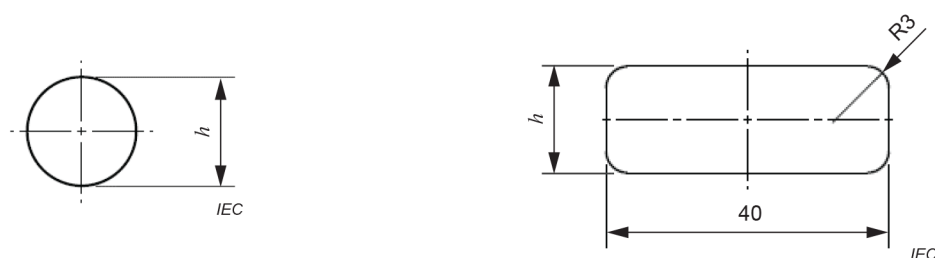
Figure 26 – Drawings of cylindrical and rectangular thresholds
