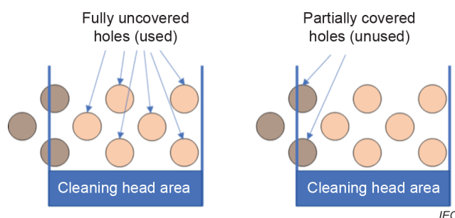
Figure 4 – Large debris template hole alignment
