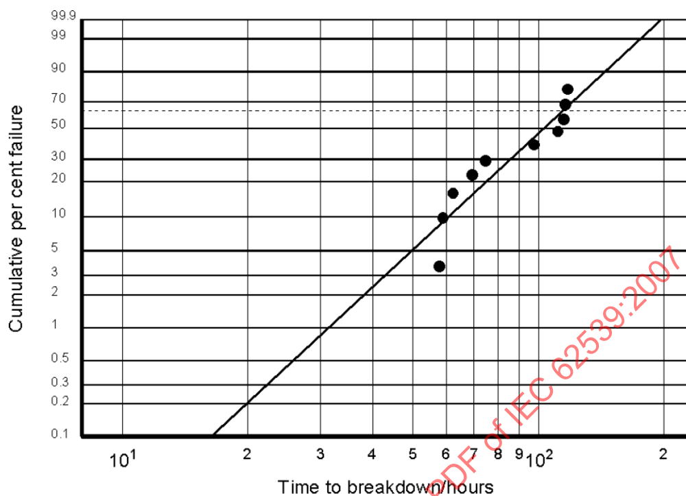
Figure A.5—Weibull plot of PET data presented in Table A.3
