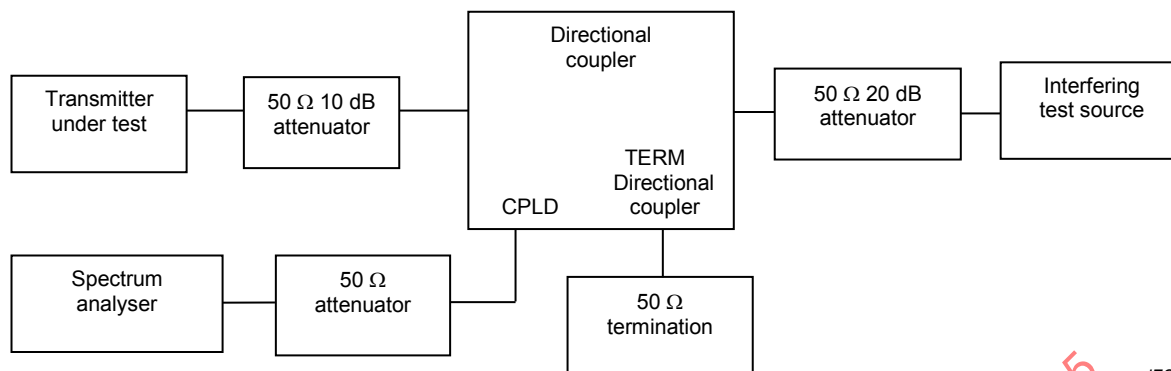
Figure 12 – Measurement arrangement for intermodulation attenuation
