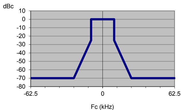
Figure 3 – Modulation spectrum for slotted transmission
