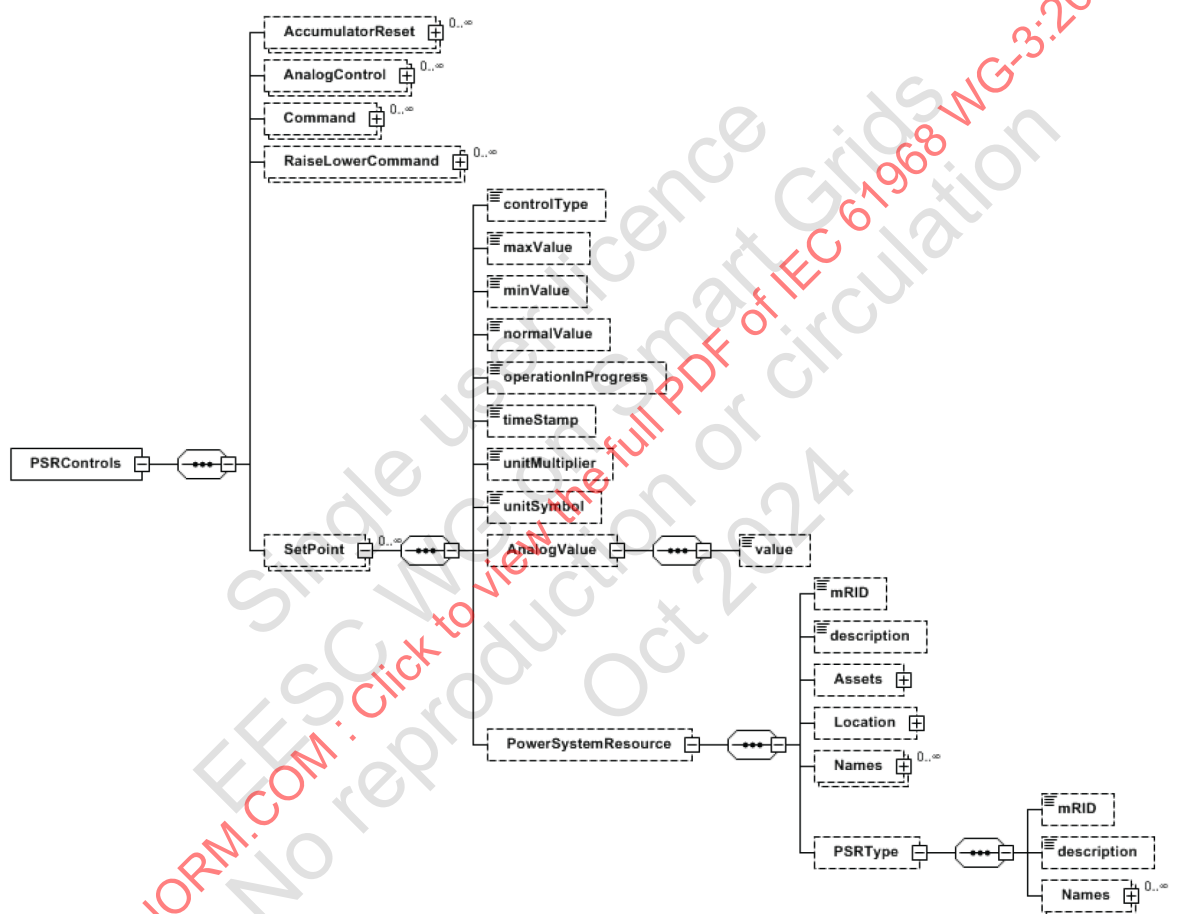
Figure 24 – PSRControls payload SetPoint
