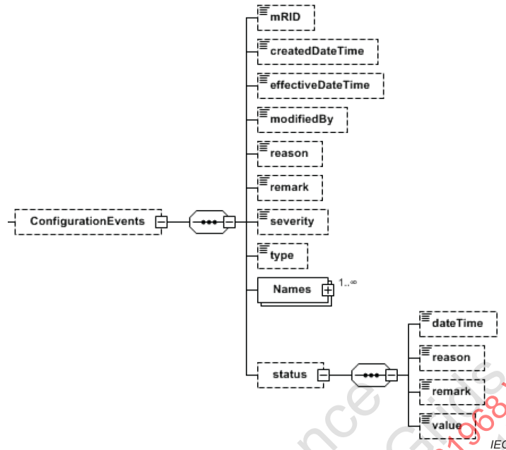
Figure B.4 – ConfigurationEvent payload fragment
