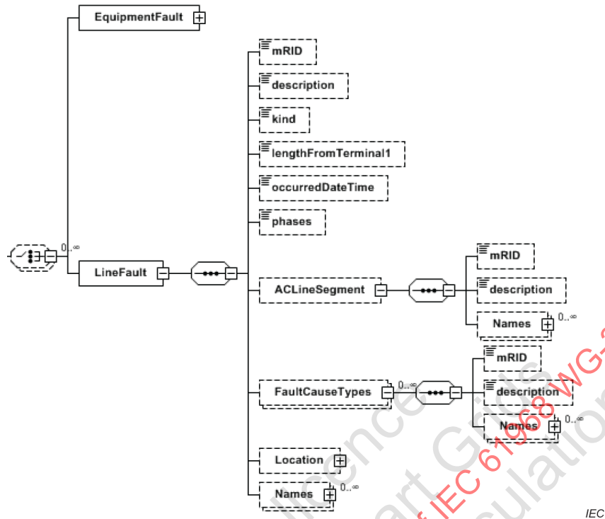
Figure 105 – TroubleOrders, UnplannedOutage, LineFault payload fragment
