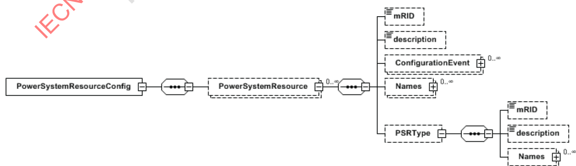
Figure 9 – PowerSystemResourceConfig payload
