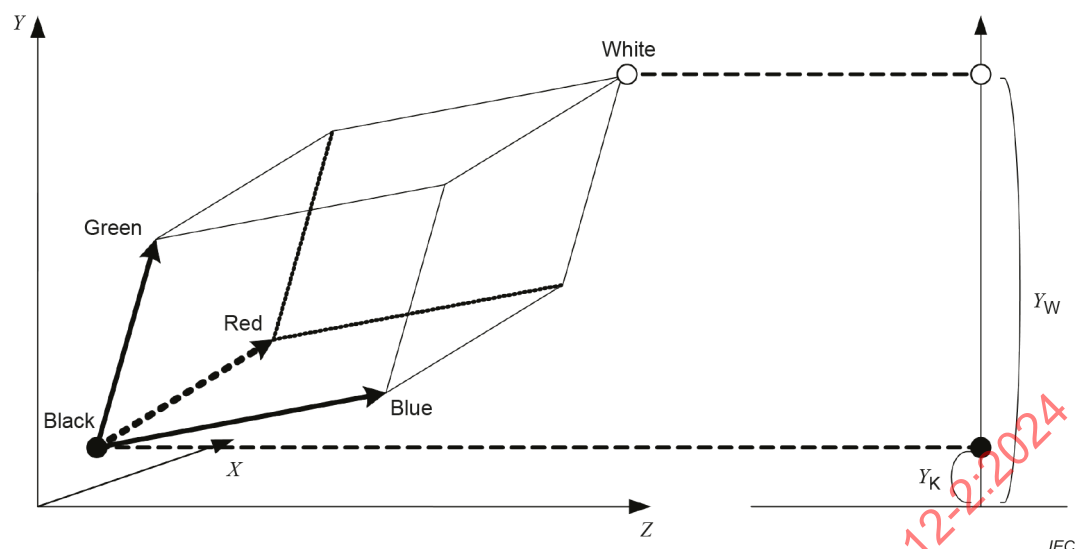
Figure 1 – The colour gamut for display types comprising three primary additive colours
