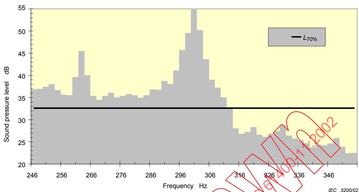
Figure 8 – Illustration of L_{70\%} level in the critical band
