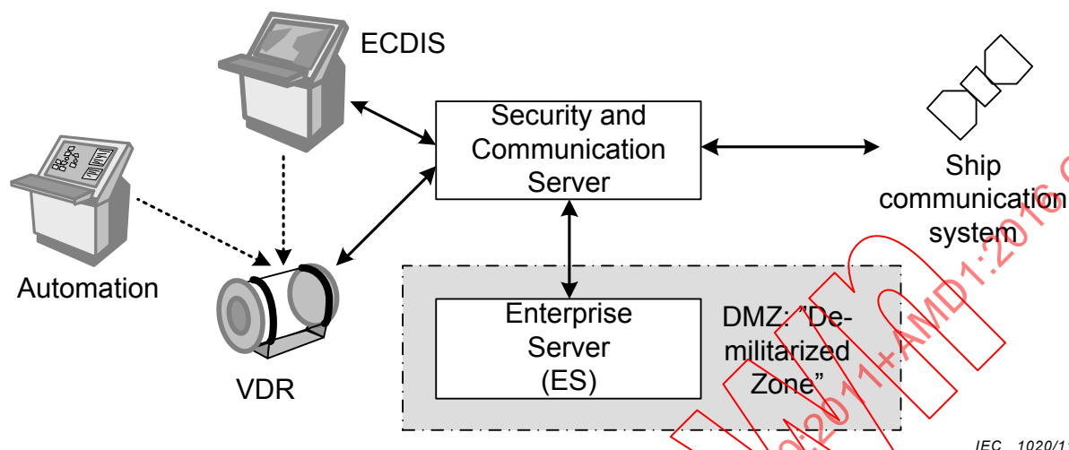
Figure D.3 – Security infrastructure
