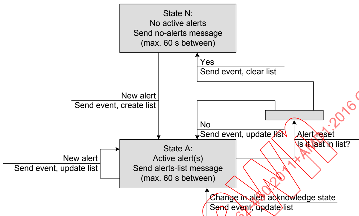
Figure C.2 – State diagram
