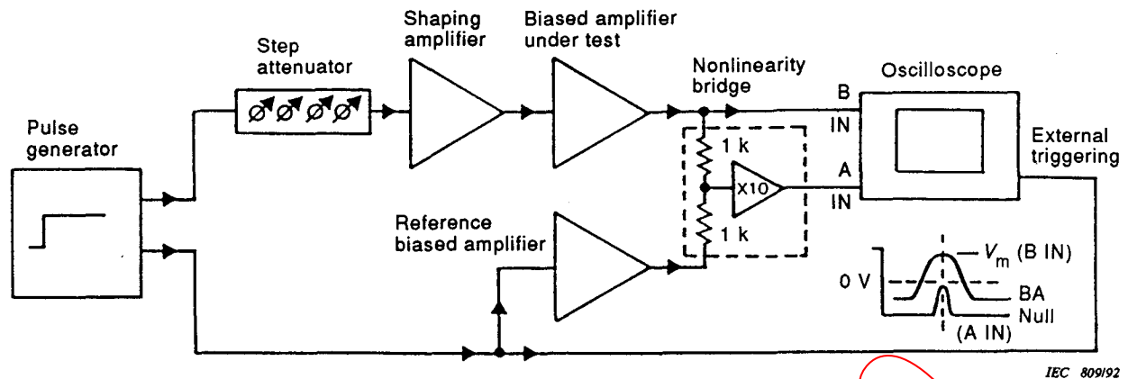
Figure 11 - Test set-up for measuring nonlinearity of a biased amplifier
