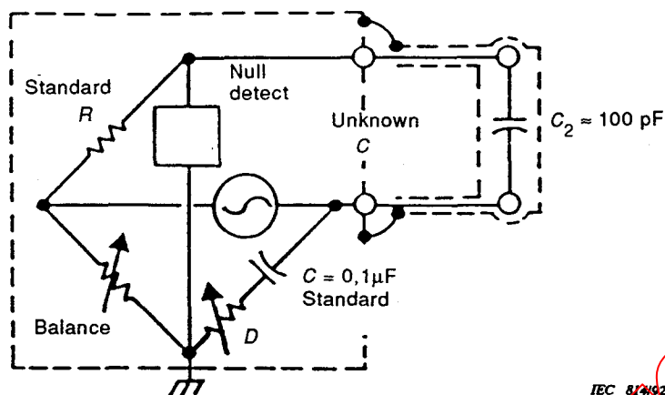
Figure B.2 - Capacitance bridge
