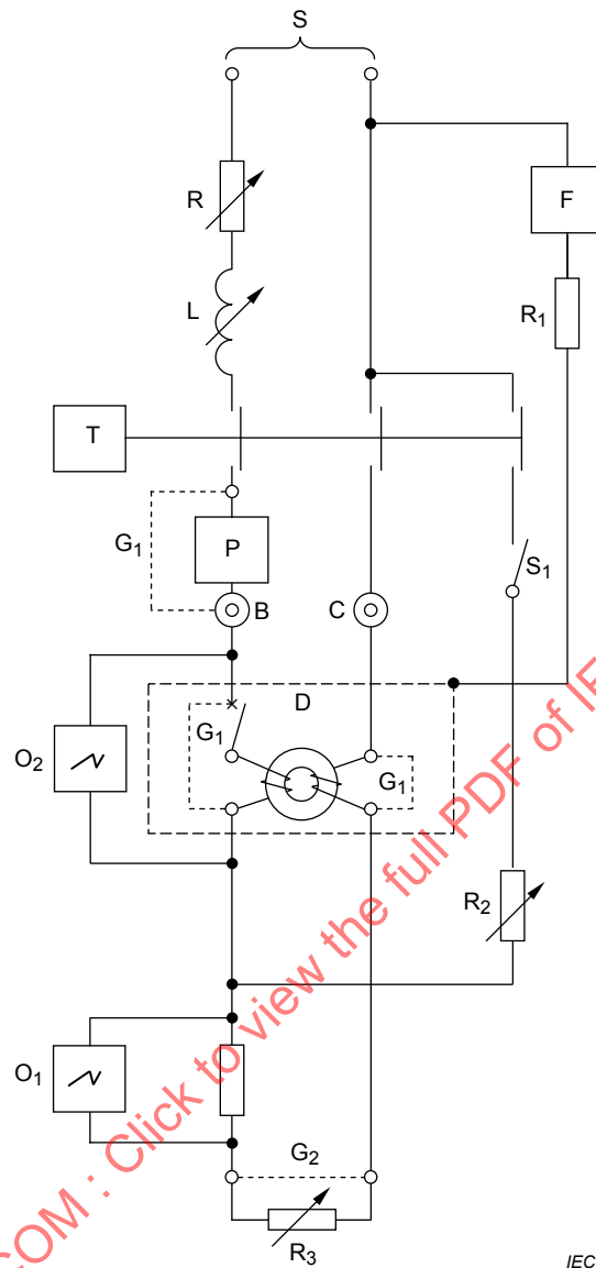
Figure 8 – Test circuit for the verification of the rated making and breaking capacity and of the coordination with a SCPD of a single-pole RCCB with two current paths (9.11)
