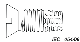
Figure 2 – Thread cutting tapping screw (3.6.11)
