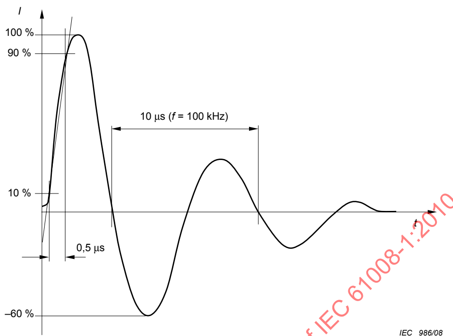
Figure 23 – Current ring wave 0,5 \mu\text{s} /100 kHz
