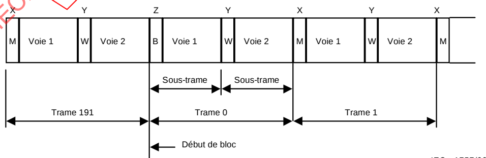
Figure 2 – Format de la trame
