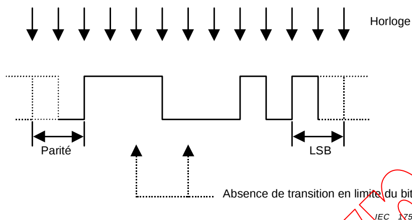
Figure 4 – Préambule M (11100010)
