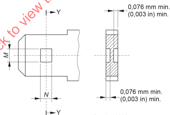
Section Y-Y
