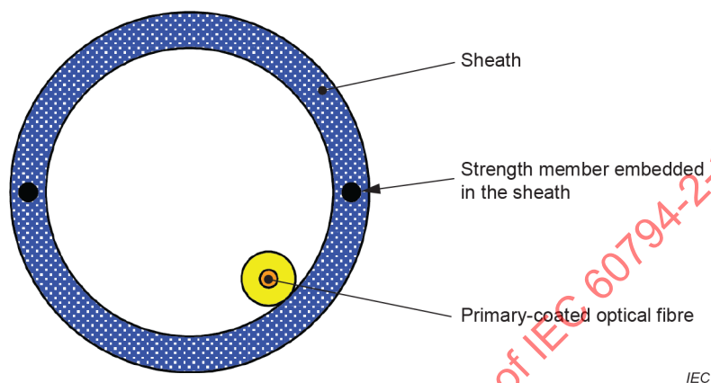
Figure A.1 – Simplex loose non-buffered fibre cable
