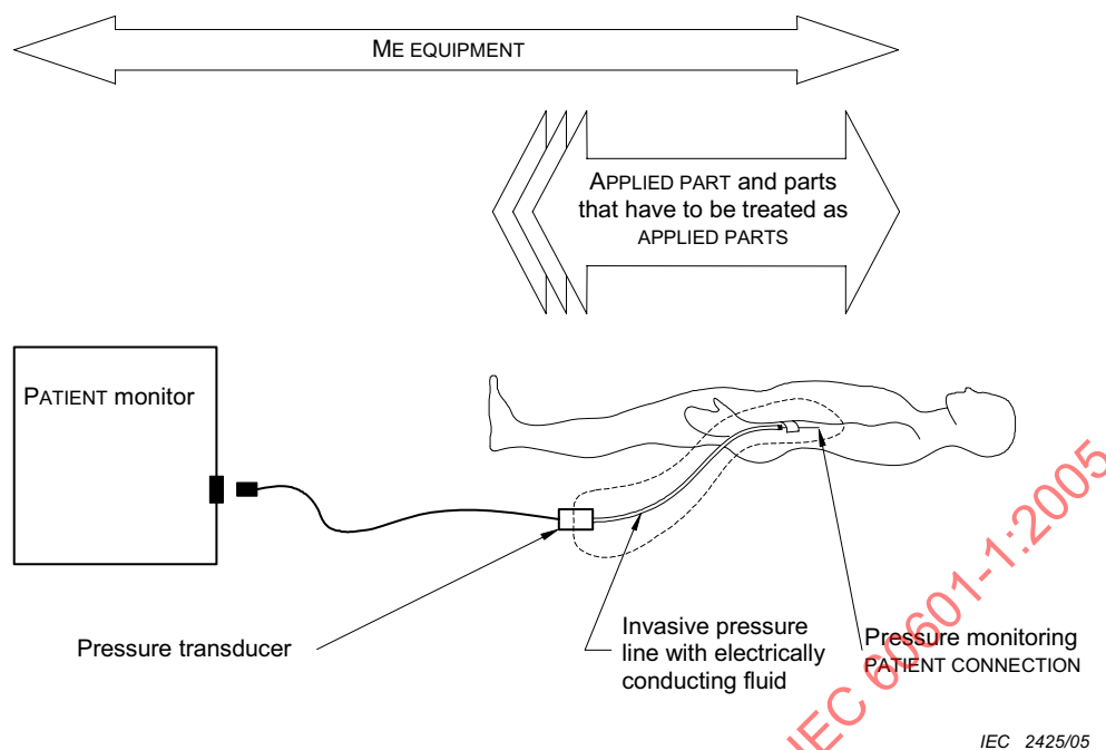
Figure A.3 – Identification of ME EQUIPMENT, APPLIED PARTS and PATIENT CONNECTIONS in a PATIENT monitor with invasive pressure monitoring facility
