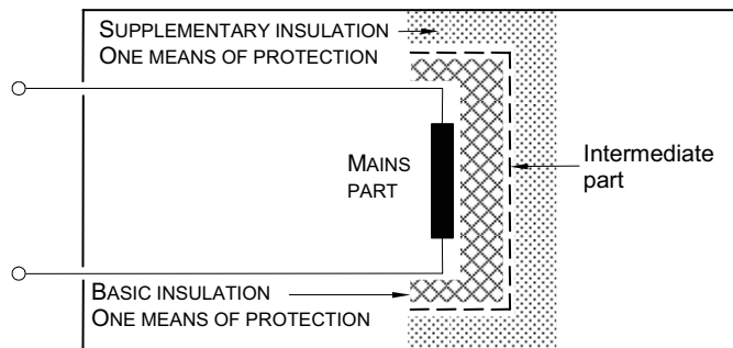
Figure J.3 – Insulation example 3
