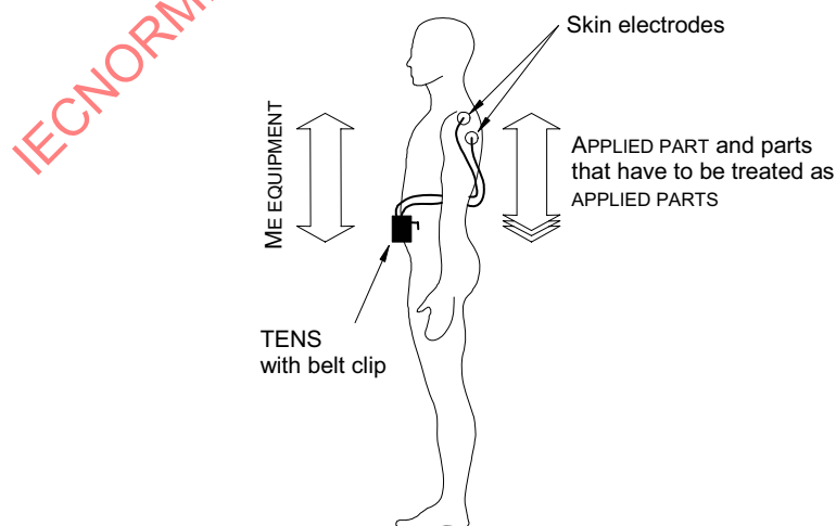
Figure A.6 – Identification of ME EQUIPMENT, APPLIED PARTS and PATIENT CONNECTIONS in a transcutaneous electronic nerve stimulator (TENS) intended to be worn on the PATIENT's belt and connected to electrodes applied to the PATIENT's upper arm
