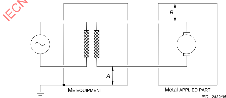
Figure A.10 – Floating circuit
