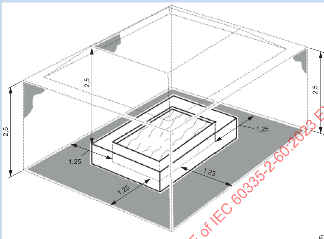
Figure 101 – Installation zone dimensions for transportable whirlpool spas
