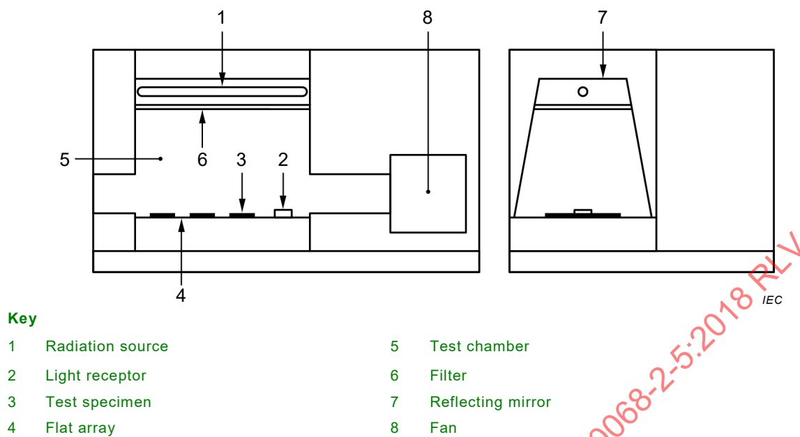
Figure C.2 – Example of test apparatus with flat array
