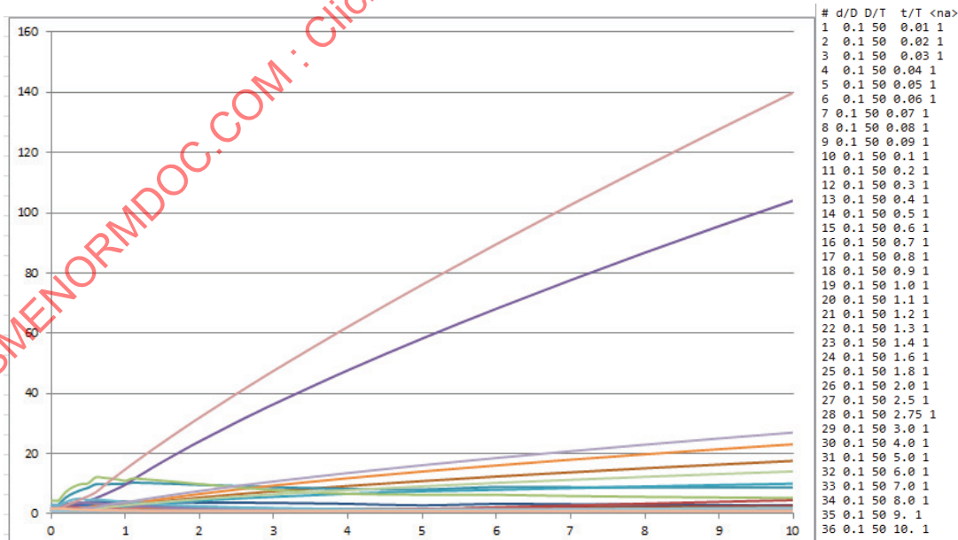
Plot 1-1 – Low d/D and D/T All Stress Factors as a Function of t/T ; d/D=0.1 ; D/T=50 ; t/T=\text{varying}
