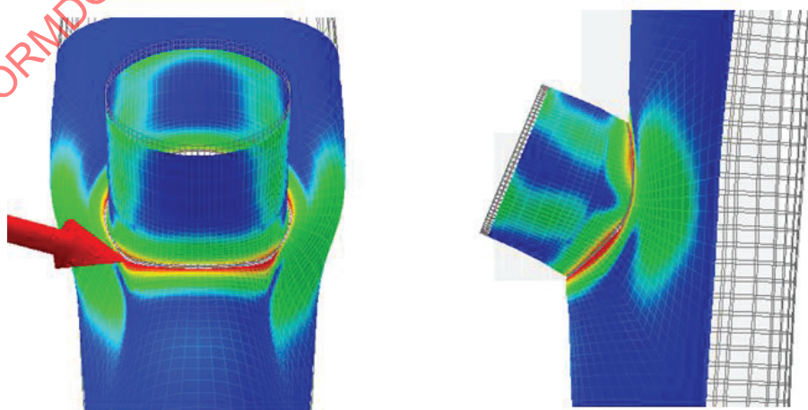
Figure 4-6: Stress Distribution Due to In-Plane Bending Moment
