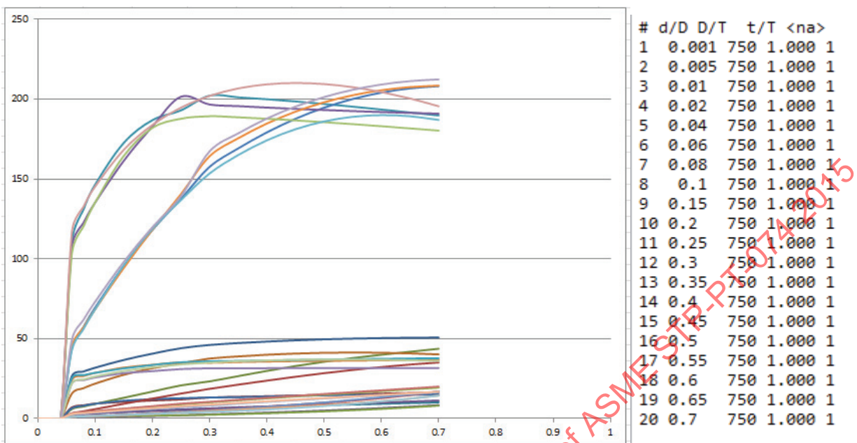
Plot 1-17 – Varying d/D ; D/T=750 ; t/T=1.0
