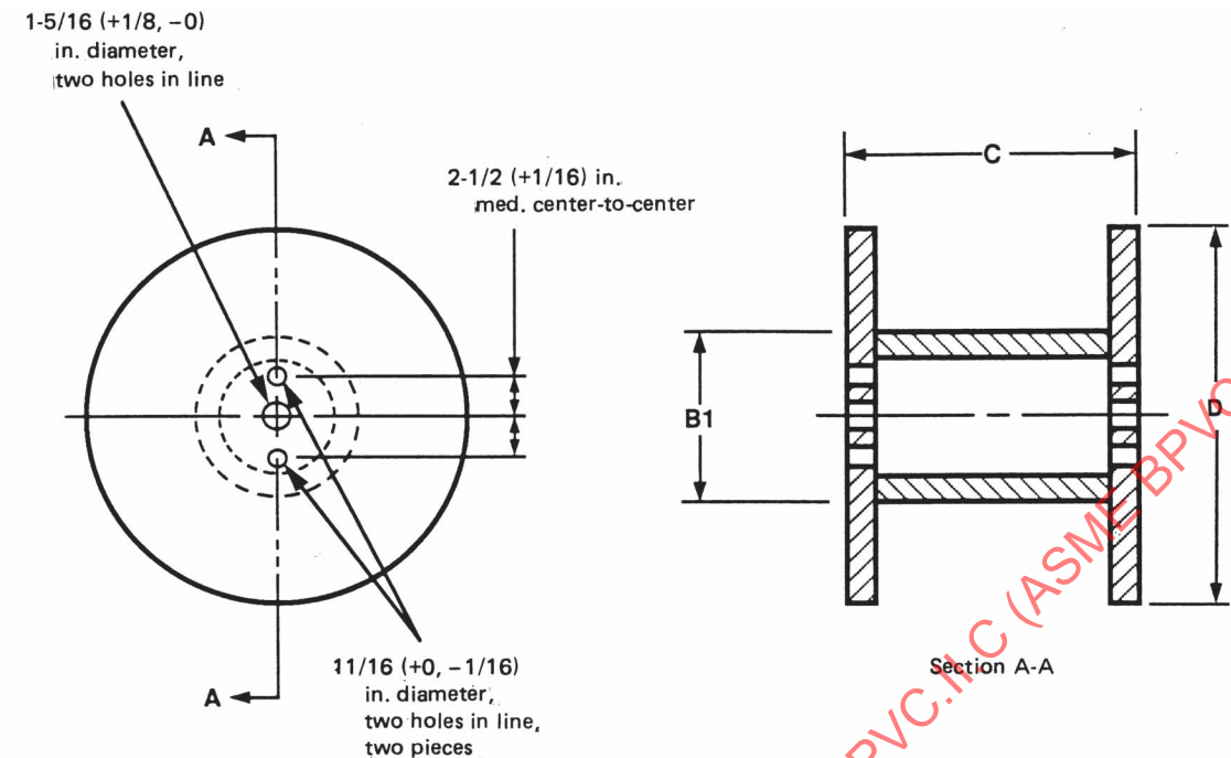
FIG. 3 DIMENSIONS OF 30 IN. (760 MM) SPOOLS
