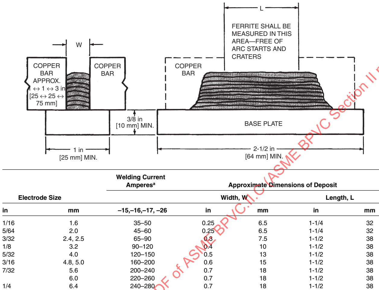
Figure A.1—Weld Pad for Ferrite Test
